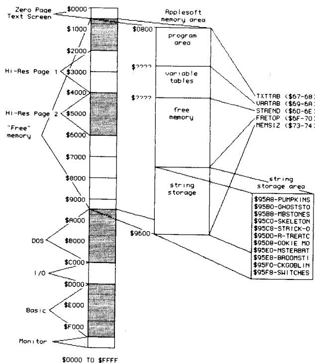
Figure 1. Applesoft string storage
